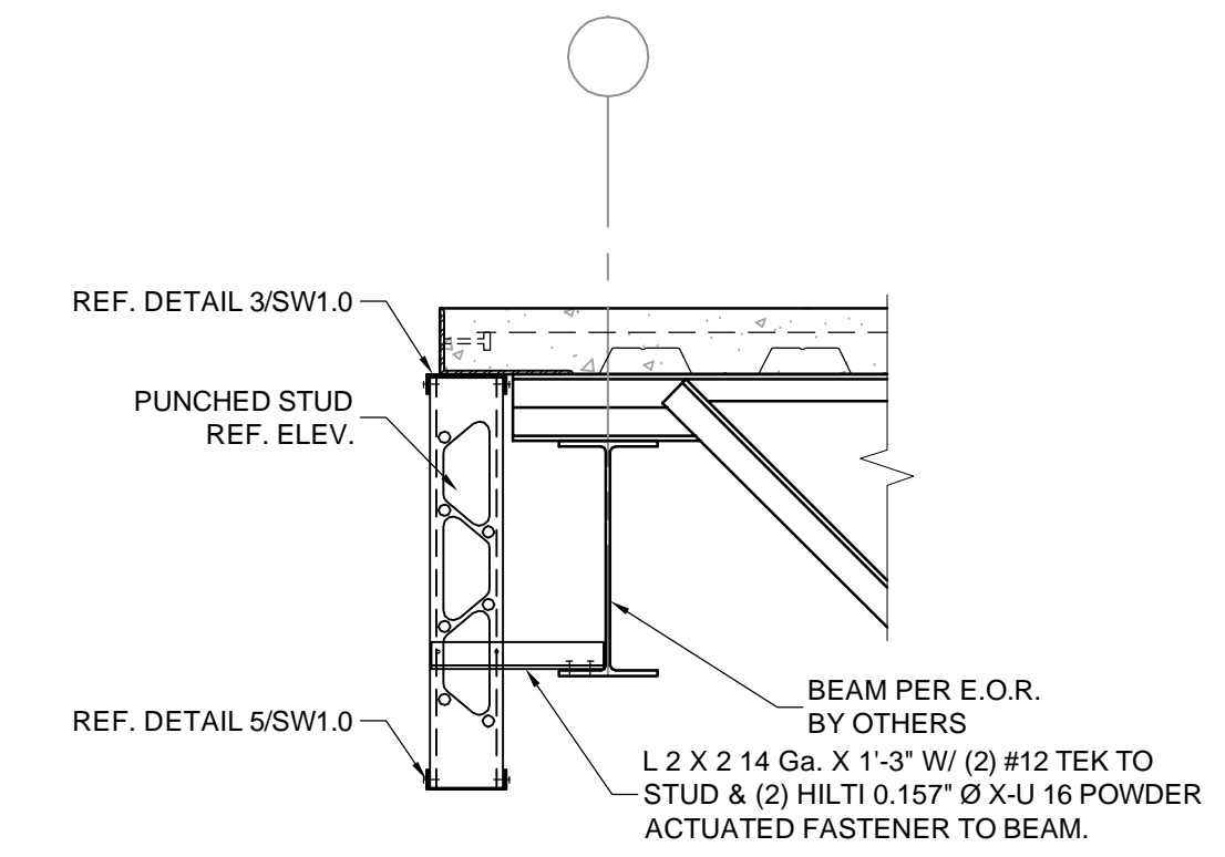
5 BALCONY @ BEAM N.T.S. 2/S-302
