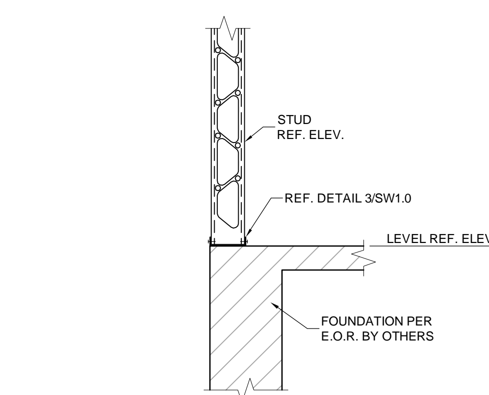
16 WALL TO FOUNDATION N.T.S.
