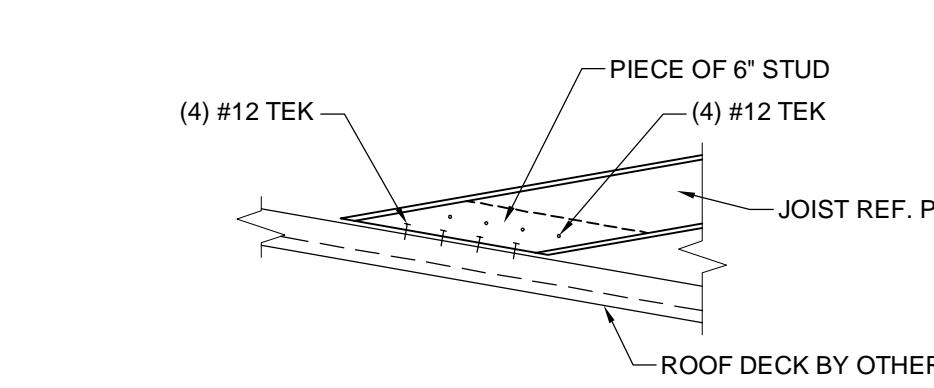
12 JOIST AT VALLEY N.T.S.
