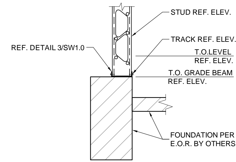
1 WALL @ GRADE BEAM N.T.S.
