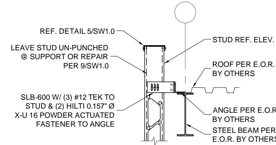
8 WALL TO ROOF N.T.S.
