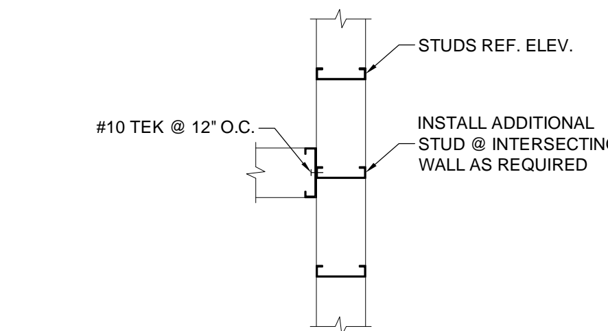
11 WALL INTERSECTION N.T.S. 2/S-503
