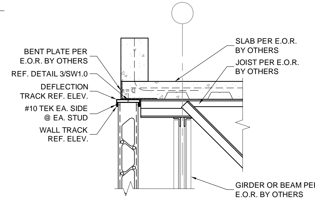
4 TRACK TO SLAB N.T.S. 4/S-404
